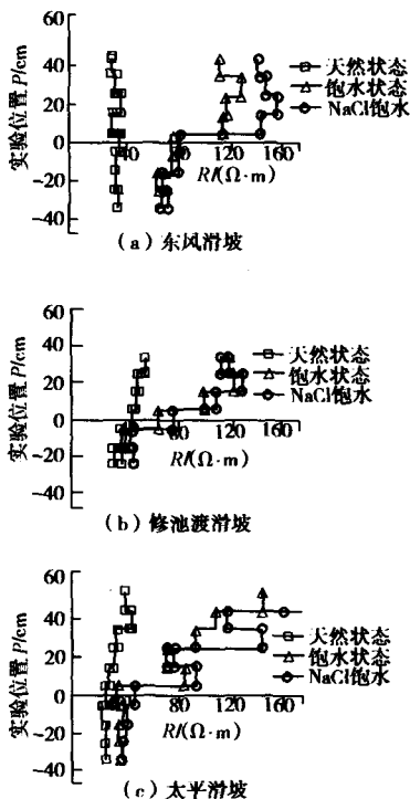
图 4 物探成果 P-R(\Omega) 关系曲线 Fig. 4 Relationship between P and R
